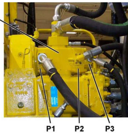
TRIPLE PUMP
